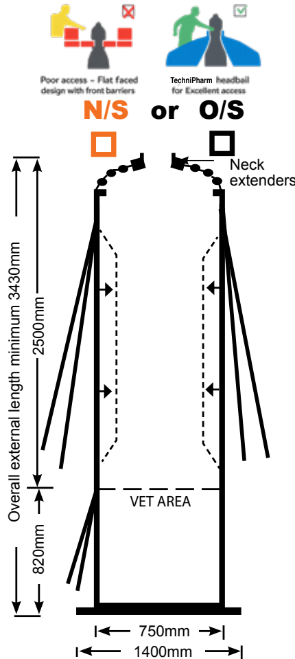
TechniPharm – Cattle Handler- New Generation Farm Ready Specifications
