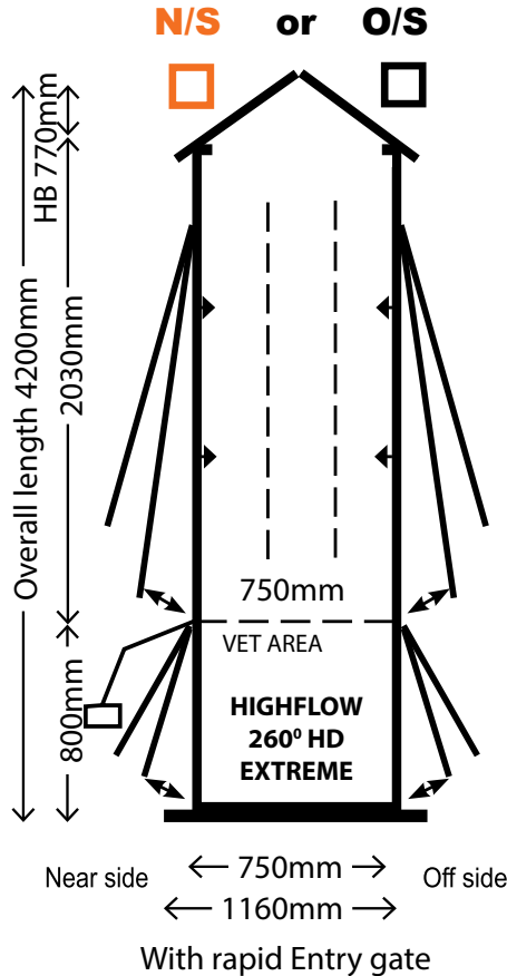
TechniPharm – Cattle Handler- New Generation Farm Ready Specifications
